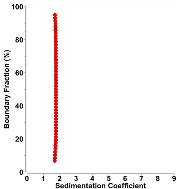
SI 7: Integral sedimentation coefficient distribution for MT-II in LPPG. Blue: 26 \mu M, red: 52 \mu M.
