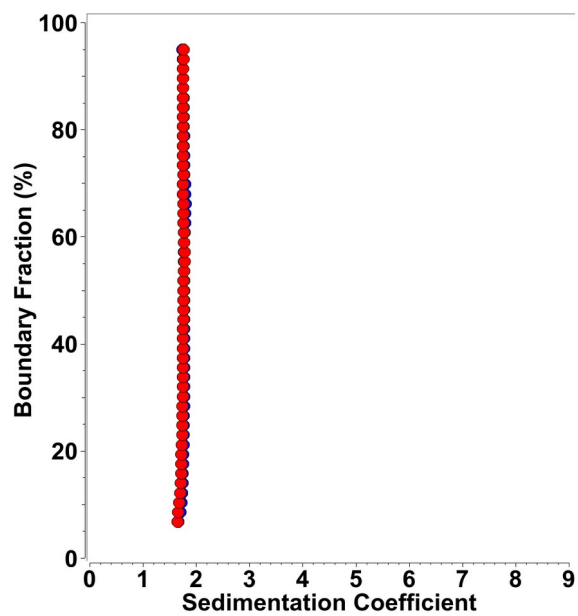
SI 9: Integral sedimentation coefficient distribution for MT-II in LSPG. Blue: 26 \mu\text{M} , red: 52 \mu\text{M} .
