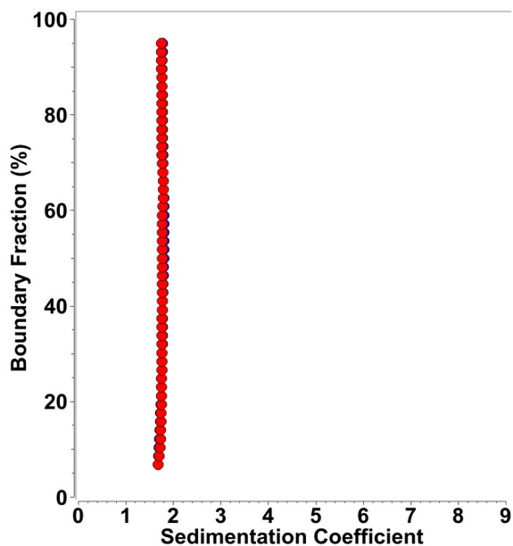
SI 8: Integral sedimentation coefficient distribution for MT-II in LPPC. Blue: 26 \mu M, red: 52 \mu M.
