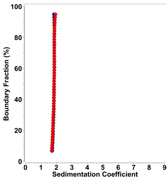
SI 6: Integral sedimentation coefficient distribution for MT-II in LMPG. Blue: 26 \mu M, red: 52 \mu M.
