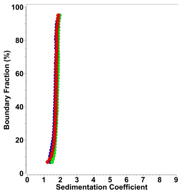
SI 5: Integral sedimentation coefficient distribution for MT-II in D310LA. Blue: 0.6 mM, green: 1.2 mM, red: 26 \mu M.
